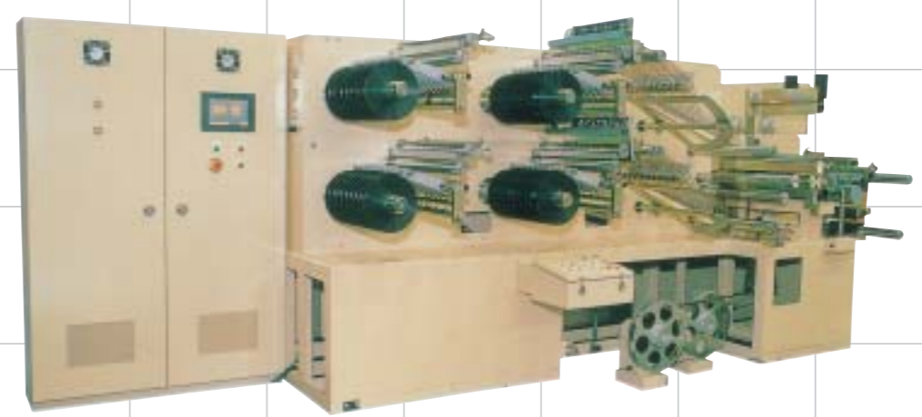
For SEMICONDUCTOR DEVICE PI FILM SLITTER MODEL 731A
